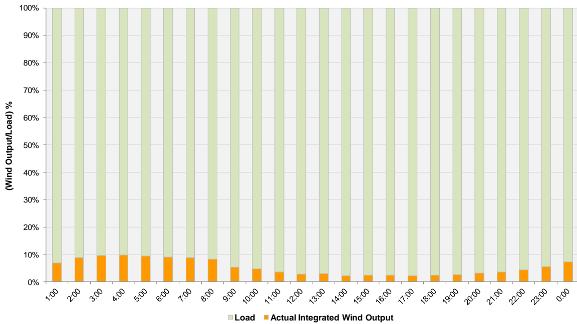
Actual Wind Output as a Percentage of the ERCOT Load 08-02-2011
