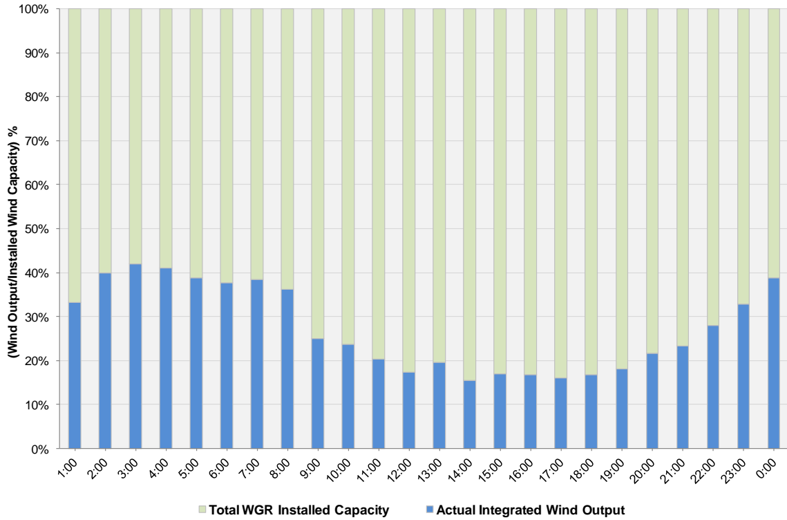
Actual Wind Output as a Percentage of the Total Installed Wind Capacity 08-02-2011
